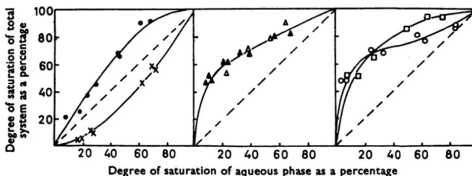
Figure 7.40 Distribution of hexachlorophene in solutions of various agents in aqueous 0.05M tris buffer, pH 8.0 at 25° C. ○, sucrose laurate 1%. □, polysorbate 20 1%. △, lauromacrogol 0.1%. ▲, lauromacrogol 1%. ×, macrogol 1%. ●, poloxamer 188 1%. Lauromacrogol = Brij 35; macrogol = PEG 4000; sucrose laurate = sucrose mono-laurate; poloxamer 188 = Pluronic F68.
