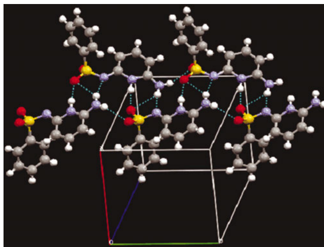
Figure 4 Packing diagram for VI. Selective view showing the hydrogen bonding scheme, mediated by a screw axis along b . Note that all H donors are satisfied, and all acceptors have at least one H contact.
