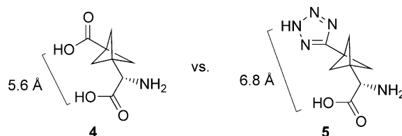
Figure 2. The size of tetrazole 5 extends the distance between the two acidic pharmacophores relative to the analogous dicarboxylic acid 4 .
