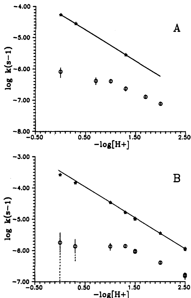
Figure 1. Plots of \log k_{hyd} (*) and \log k_{ex} (O) vs. -\log [H_3O^+] for N -cyclohexylacetamide (A) and acetanilide (B) determined at 100 and 72 °C, respectively, \mu = 1.0 M KCl. The k_{ex} values are calculated from percent ^{18}O content at t_{1/2} hydrolysis (see text). Dashed error bars in exchange data of B indicate there is no satisfactory lower limit due to error limits exceeding the value of k_{ex} . Straight lines through k_{hyd} data are unit slope first-order dependence on [H_3O^+] .
