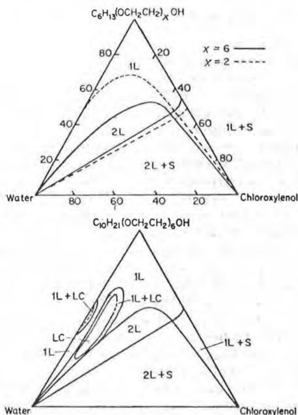
Figure 6.1 The upper phase diagram (after Mulley and Metcalf [12]) illustrates the phases existent in the system C_6H_{13}(OCH_2CH_2)_xOH : 4-chloro-3,5-xylenol: water at 20°C. The dotted line represents the behaviour when x = 2 and the solid lines where x = 6 . The lower diagram shows the much more complex behaviour in the system: C_{10}H_{21}(OCH_2CH_2)_6OH : chloroxylenol: water. 1L = isotropic liquid; LC = liquid crystalline; S = solid 2L = two liquids (immiscible.)
