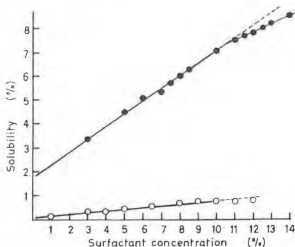
Figure 6.13 Solubility of chlorhexidine diacetate (●) and dihydrochloride (○) as a function of concentration of the decaoxyethylene oleic ether, Brij 96. Each point is the average of two or three independent determinations. From Wesoluch et al. [66] with permission.
