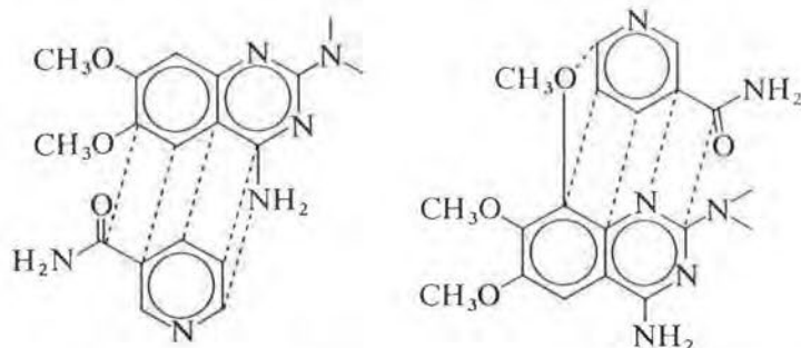
Schematic representation of interaction between niacinamide and (XXXI) and (XXXII) from Fawzi et al. [300] with permission.
