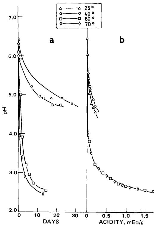
Figure 3 —The pH change of 3% aqueous polysorbate 20 at 70, 60, 40, and 25° in daylight with no catalyst, with time (a), and as a function of total acidity at the corresponding time (b).
