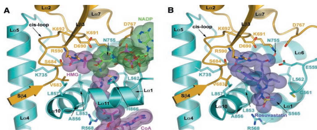
Fig. 2. Statins exploit the conformational flexibility of HMGR to create a hydrophobic binding pocket near the active site. (A) Active site of human HMGR in complex with HMG, CoA, and NADP. The active site is located at a monomer-monomer interface. One monomer is colored yellow, the other monomer is in blue. Selected side chains of residues that contact the substrates or the statin are shown in a ball-and-stick representation (20). Secondary structure elements are marked by black labels. HMG and CoA are colored in magenta; NADP is colored in green. To illustrate the molecular volume occupied by the substrates, transparent spheres with a radius of 1.6 Å are laid over the ball-and-stick representation of the substrates or the statin. (B) Binding of rosuvastatin to HMGR. Rosuvastatin is colored in purple; other colors and labels are as in (A). This figure and Figs. 3 and 4 were prepared with Bobscript (22), GLR (23), and POV-Ray (24).
