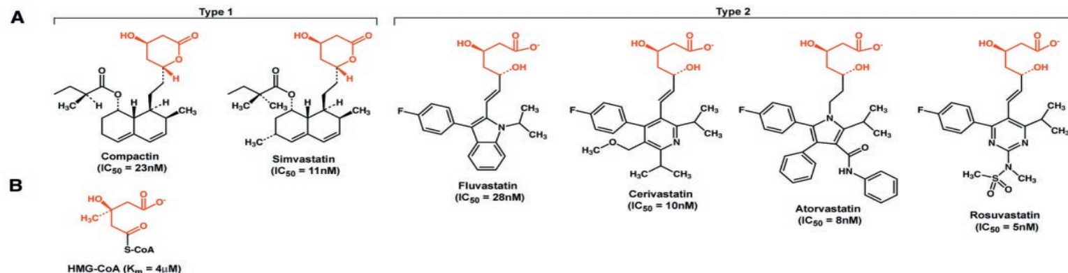
Fig. 1. Structural formulas of statin inhibitors and the enzyme substrate HMG-CoA. (A) Structure of several statin inhibitors. Compactin and simvastatin are examples of type 1 statins; not shown are the other type 1 statins, lovastatin and pravastatin. Fluvastatin, cerivastatin, atorvastatin, and
