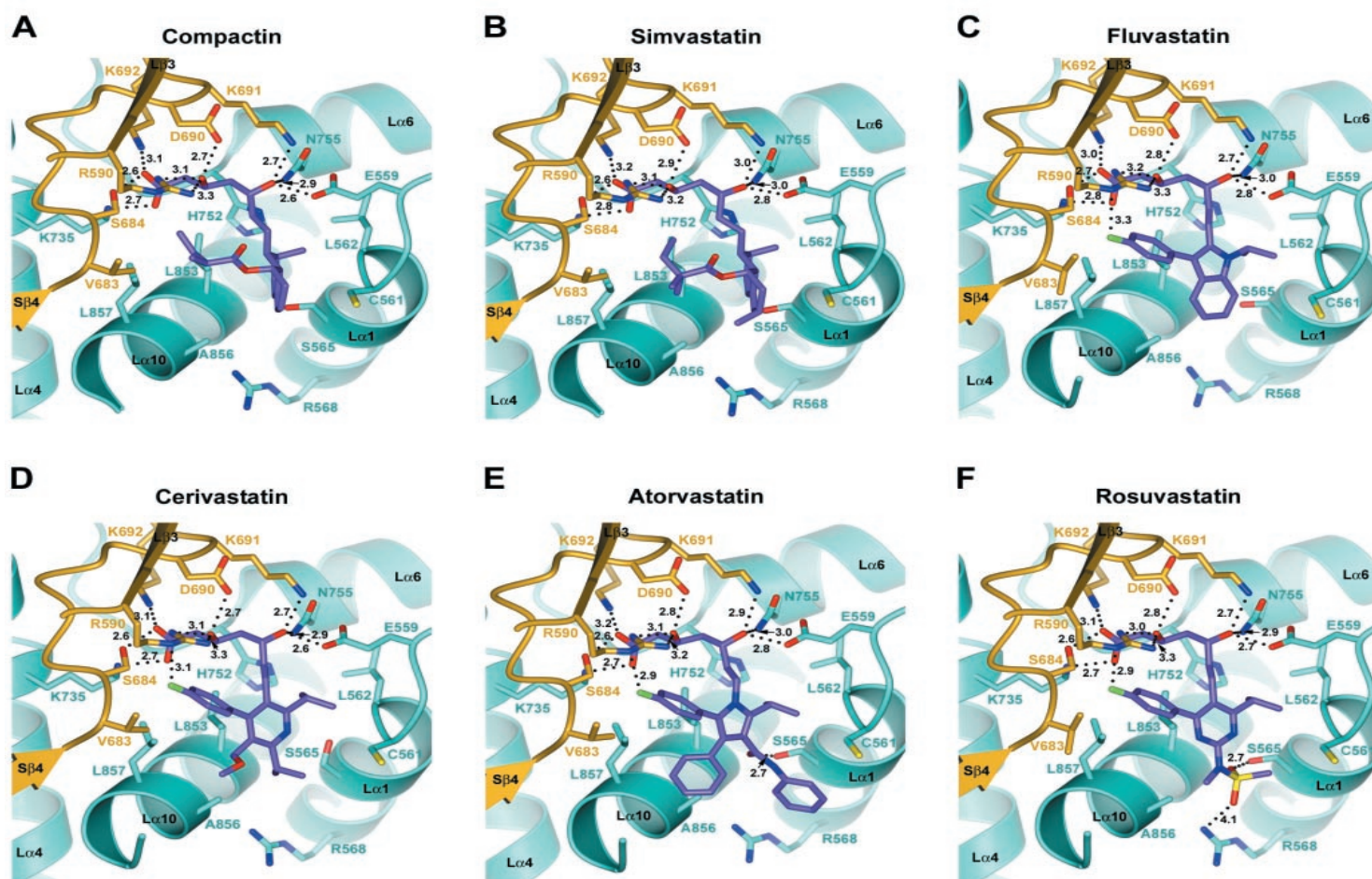
Fig. 4. Mode of binding of compactin (A), simvastatin (B), fluvastatin (C), cerivastatin (D), atorvastatin (E), and rosuvastatin (F) to human HMGR. Interactions between the HMG moieties of the statins and the protein are mostly ionic or polar. They are similar for all inhibitors and are indicated by the dotted lines. Numbers next to the lines indicate distances in Å (13). The rigid hydrophobic groups of the statins are
