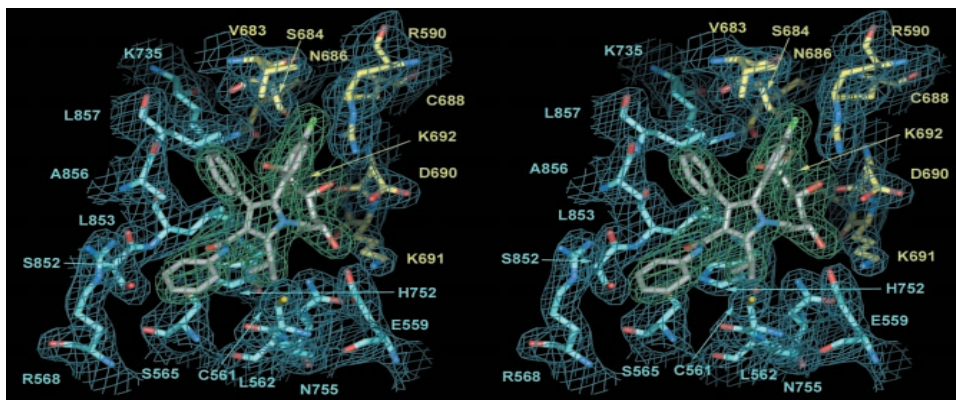
Fig. 3. Stereoview of the electron-density map of atorvastatin bound to the HMGR active site. This 2.2 Å simulated-annealing omit map, contoured at 1 \sigma , was calculated by omitting all atoms of the atorvastatin molecule shown, as well as protein atoms within 4.5 Å of the inhibitor. The electron density is overlaid on the final, refined model. The electron density covering atorvastatin is in green, whereas the electron density covering the protein is in blue. Carbon atoms of one of the two protein monomers are colored yellow, those of the neighboring monomer are in blue, and those of atorvastatin are in gray. In all molecules oxygen atoms are red, nitrogen atoms are blue, sulfur atoms are yellow, and the fluorine atoms are green.
