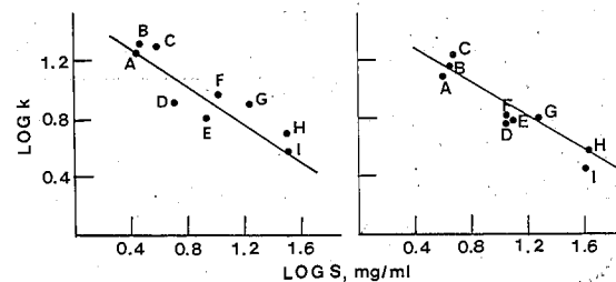
Fig. 1. Relationship between solubility in water and salting-out constant at 25°C (left) and 37°C (right). Key: A = phenazopyridine; B = cyproheptadine; C = bromhexine; D = trihexyphenidyl; E = isoxsuprine; F = chlortetracycline; G = methacycline; H = papaverine; and I = demeclocycline.
