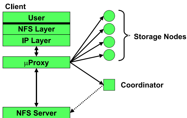
Figure 1. The Slice distributed storage architecture.
