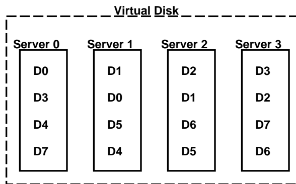
Figure 5: Chained-Declustering
