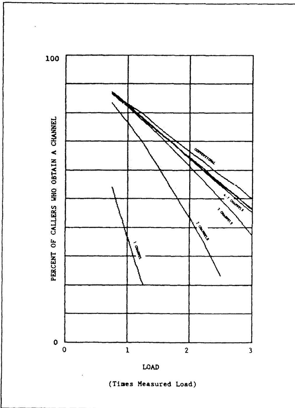
Figure 8. Percent of Callers Obtaining a Channel Within 1 Second
