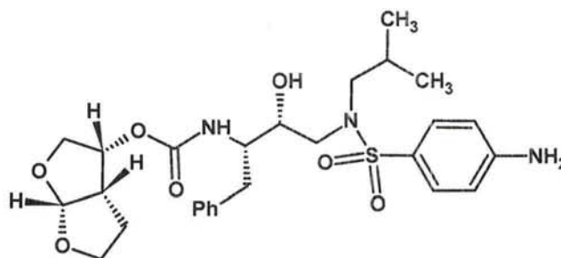
Compound 13, Darunavir
