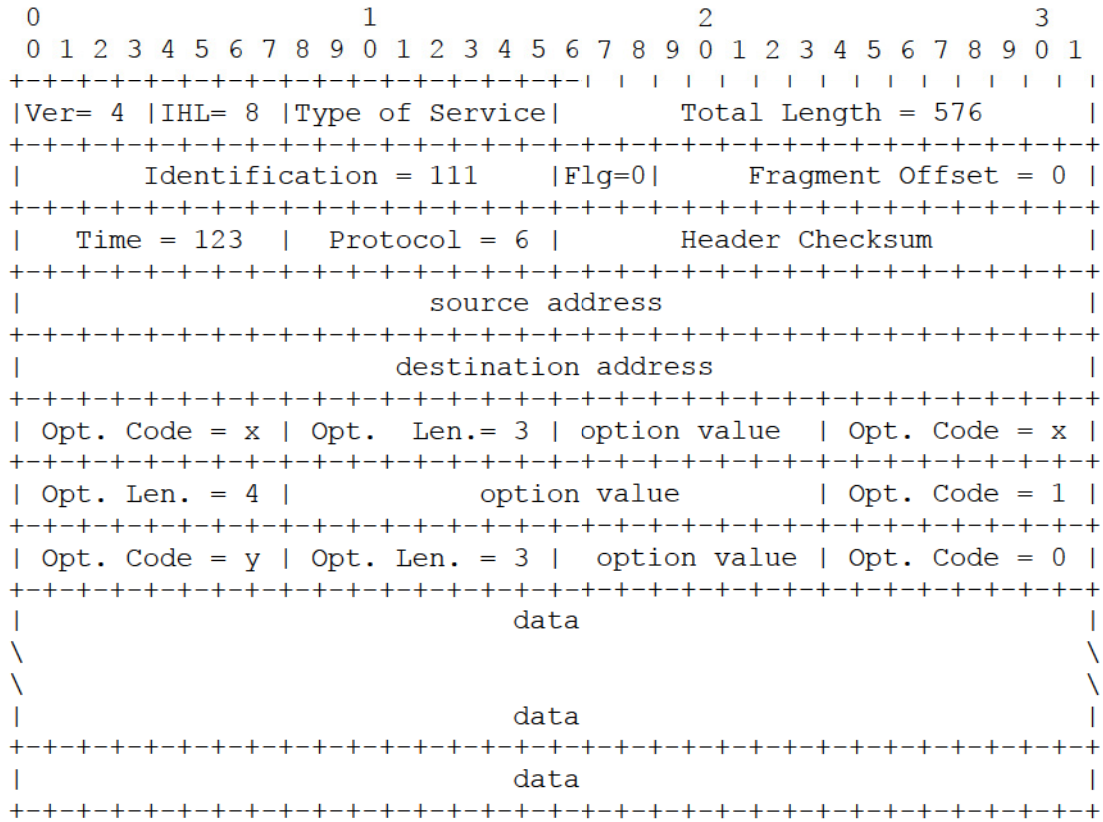
Example Internet Datagram
