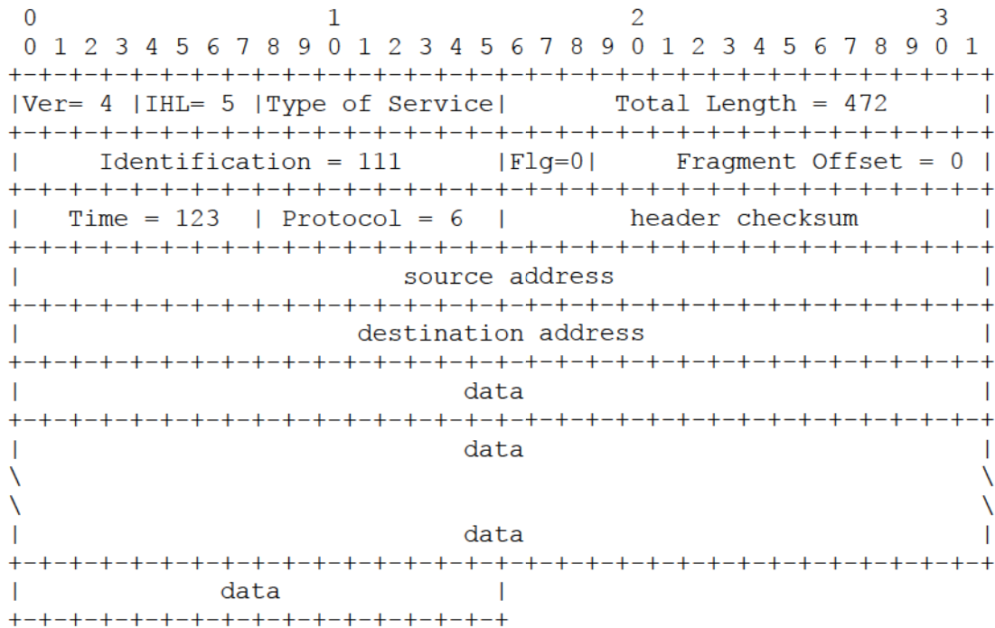
Example Internet Datagram
