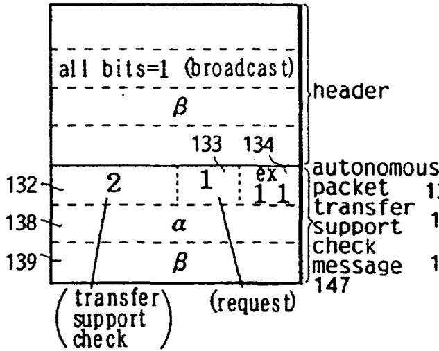
(1) data packet including message 147
