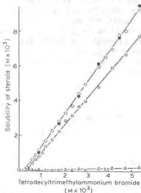
Figure 6.22 Solubility of progesterone in aqueous solutions of tetradecyltrimethylammonium bromide. \circ , progesterone only; \Delta , progesterone first and ethinyl oestradiol second; \square , ethinyl oestradiol first and progesterone second; and \bullet , progesterone and ethinyl oestradiol at the same time. From Lövgren et al. [168].
