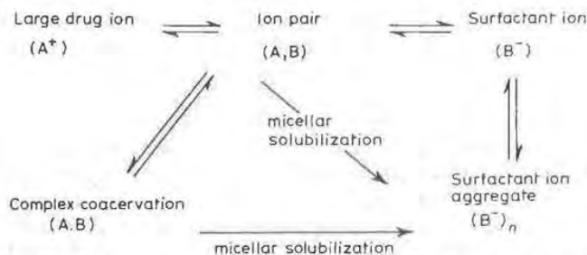
Figure 6.39 Equilibria possible in mixtures of oppositely charged organic ions when one is a surface-active agent (B - ) and the other a solute or drug molecule (A). From Tomlinson [270] with permission.
