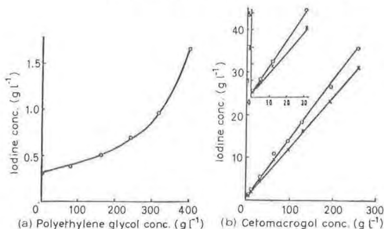
Figure 6.15 (a) The solubility of iodine in aqueous solutions of polyoxyethylene glycol 1540 at 20°C. (b) The solubility of iodine in cetomacrogol solutions at 20°C is denoted by the open circles. The available iodine is shown by the crosses; the inset shows the effect at low cetomacrogol concentrations. The much higher solubility of iodine in the detergent solutions is evident. From Hugo and Newton [77] with permission.
