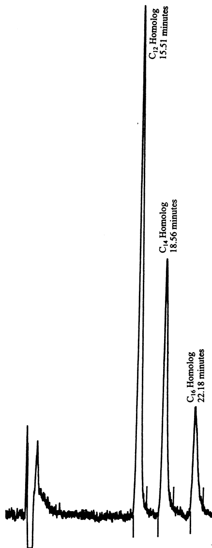
Fig. 1. Chromatogram of benzalkonium chloride 0.2 \text{ mg ml}^{-1} .
