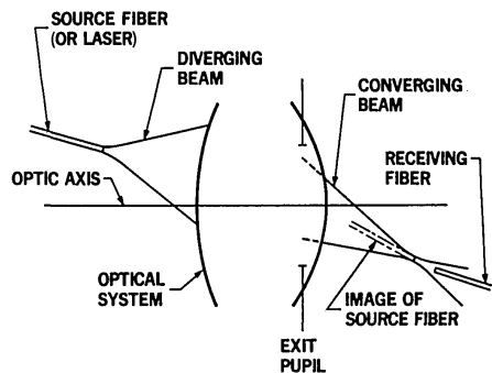
Fig. 1. Coupling from a source fiber (or laser) to a receiving fiber through a general optical system. The receiving fiber lies near an image of the source fiber.
