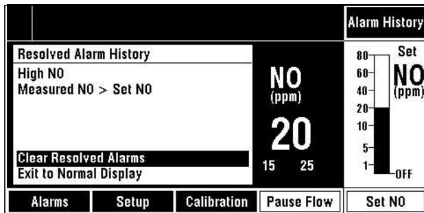
Figure 7-11 • Resolved Alarm History menu - 6 or more resolved alarms, page 2
