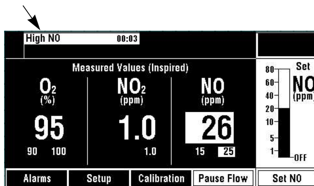
Figure 7-1 • High priority alarm message shown in most recent alarm location (upper left)
