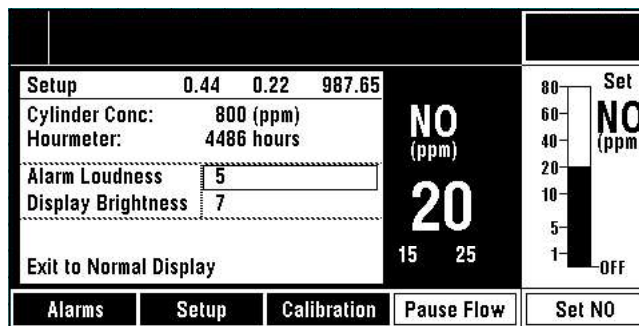
Figure 3-14 • Select menu - Alarm Loudness level selected for adjustment
