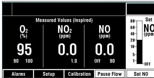
Figure 6-14 • Set NO display - normal state, NO bargraph showing 20 ppm setting
