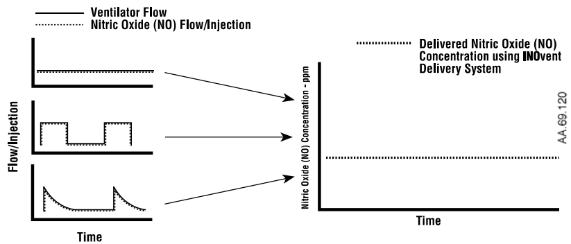
Figure 2-6 • INOvent delivery system injection method: a constant NO concentration
