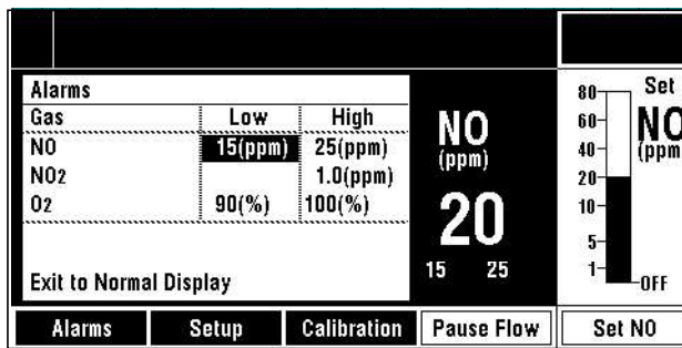
Figure 7-7 • Alarms menu - low NO alarm setting highlighted
