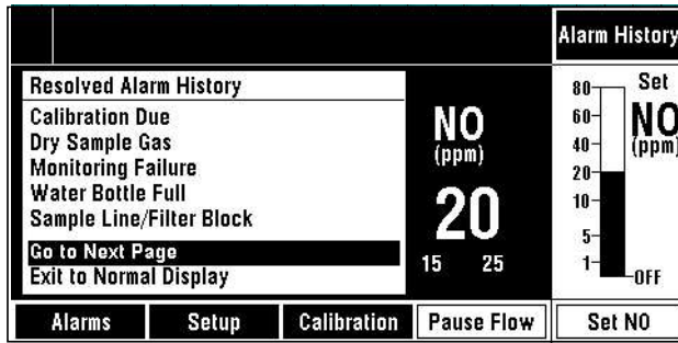
Figure 7-10 • Resolved Alarm History menu - six or more resolved alarms, page 1
