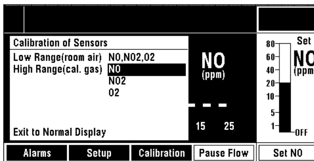
Figure 10-8 • Calibration menu - high range NO sensor calibration option highlighted
