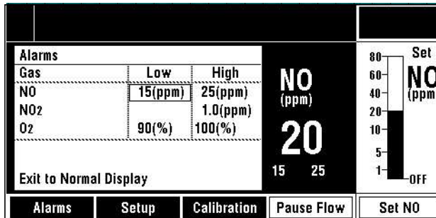
Figure 7-8 • Alarms menu - low NO alarm setting selected for adjustment
