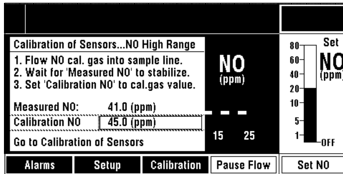
Figure 4-8 • High range calibration menu example - Calibration NO adjusted to 45 ppm
