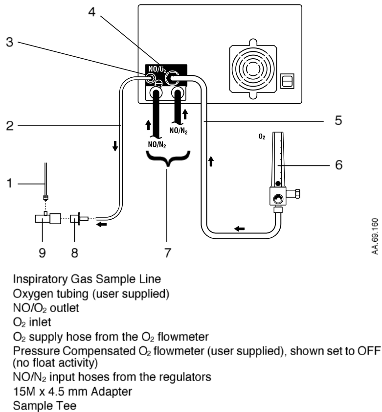
Figure 5-2 • Sample tee connection to the Manual NO delivery system
