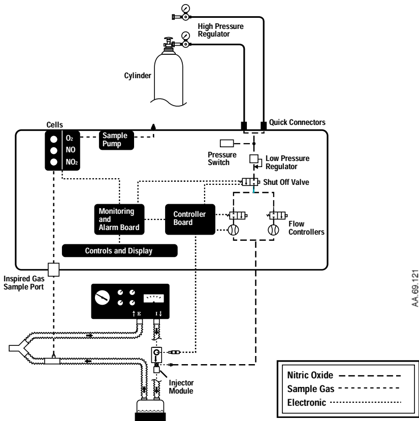
Figure 2-5 • NO Flow from the cylinder to the patient breathing circuit
