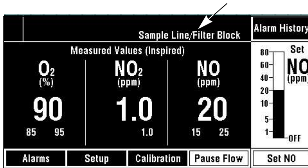
Figure 7-3 • Low priority alarm message shown in low priority alarm location
