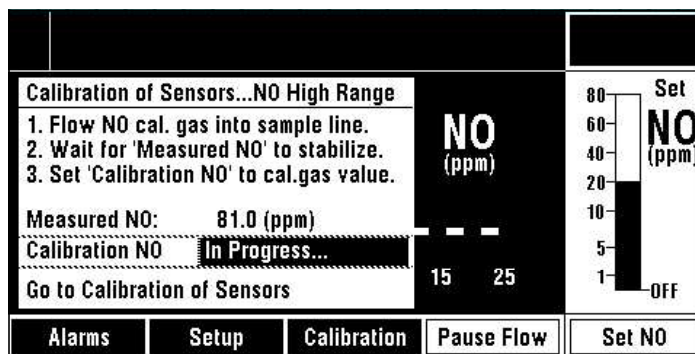
Figure 4-8 • High range calibration menu example - Calibration NO adjusted to 45 ppm
