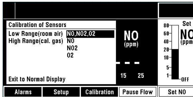
Figure 4-1 • Calibration menu - low range sensor calibration option highlighted
