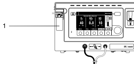
Figure 10-4 • Fluid Trap Bottle location
