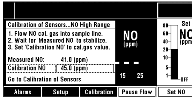
Figure 10-9 • High range calibration menu example - Calibration NO adjusted to 45 ppm
