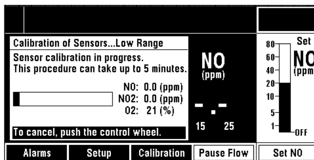
Figure 4-2 • Calibration menu - low range sensor calibration in progress
