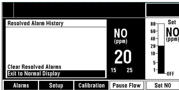
Figure 7-12 • Resolved Alarm History menu - resolved alarms cleared
