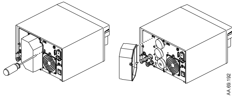
Figure 15-7 • Sensor cover removal and replacement
