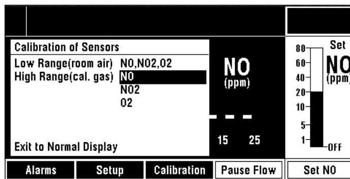
Figure 4-7 • Calibration menu - high range NO sensor calibration option highlighted
