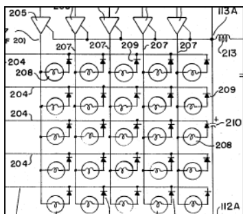
Pooley Ex. 2010 Fig. 2: incandescent lamps with rectifier diodes
