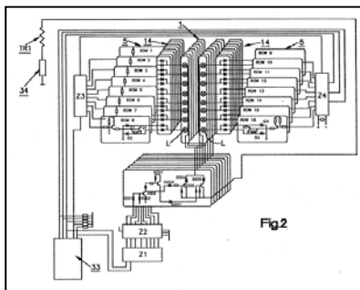
Odlen Ex. 2012 Fig. 2: AC driving circuitry for "light bulbs"
