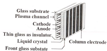
Figure 19. Schematic of a plasma addressed LCD.
