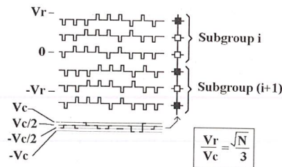
Figure 14. Illustration of row and column waveforms of multi-line addressing (IHAT, L = 3 ).
