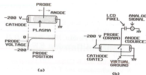
Figure 20. Principle of plasma addressing.
