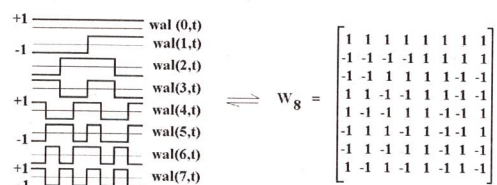
Figure 6. Walsh functions and the corresponding orthogonal matrices.
