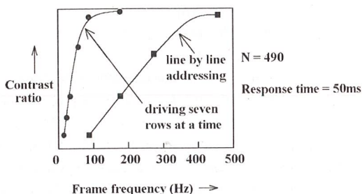
Figure 15. Contrast ratio vs frame frequency comparison between line by line and multi-line addressing.
