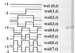
Figure 6. Walsh function orthogonal matrices.
