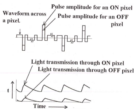
Figure 11. Frame response phenomenon associated with line by line addressing.
