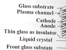
Figure 19. Schematic of plasma-addressed LCD.
