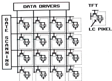
Figure 18. Active matrix LCD.
