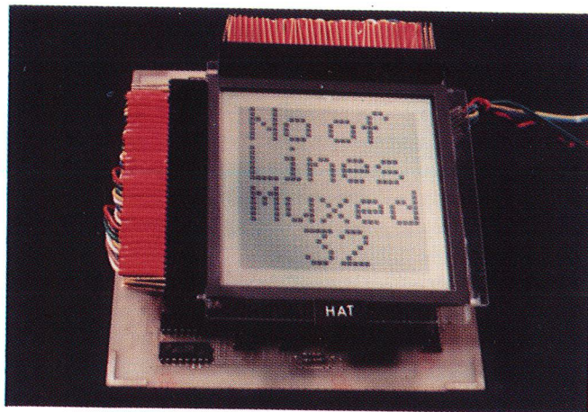
Figure 17. Photograph of a display addressed by hybrid addressing technique (a multi-line-technique) exhibits good brightness uniformity of pixels.
