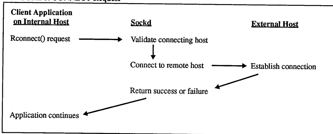
FIGURE 3. CONNECT Request
