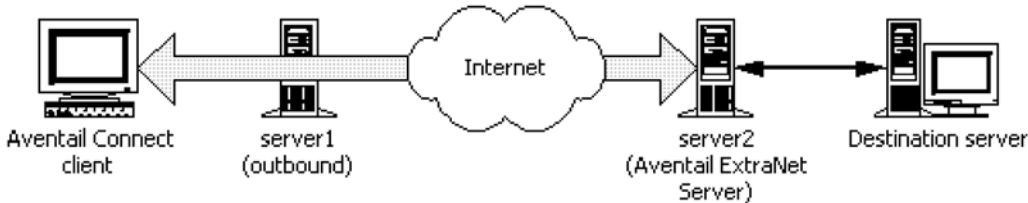
MULTIPROXY: The user authenticates with server2 directly.
