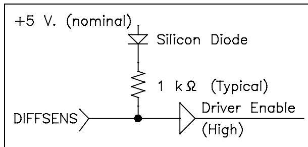
Figure 12 - Differential driver protection circuit
