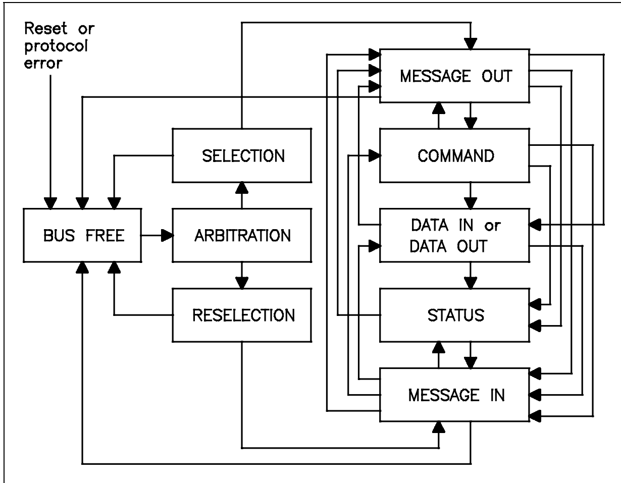
Figure 16 - Phase sequences
