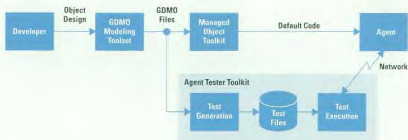
Fig. 2. Agent development and testing tools.
