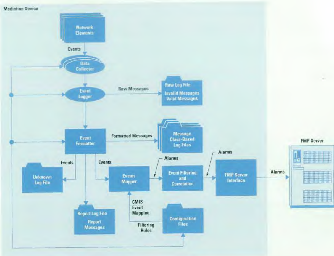
Fig. 5. Mediation device functional block diagram.
