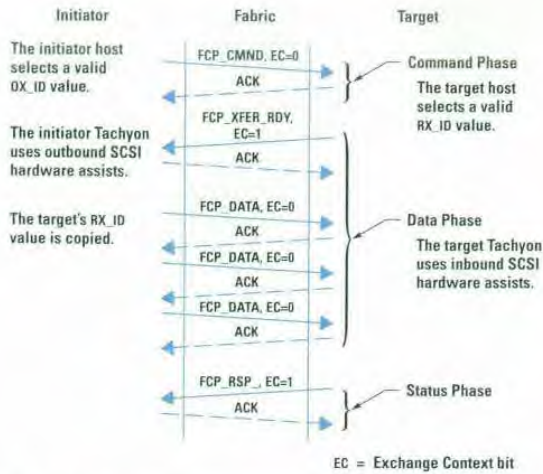
Fig. 8. FCP write exchange overview.
