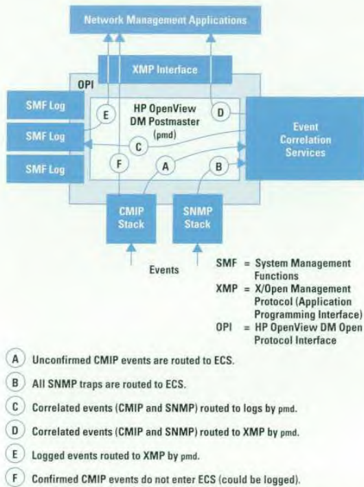
Fig. 8. Event routing to and from HP OpenView Event Correlation Services.
