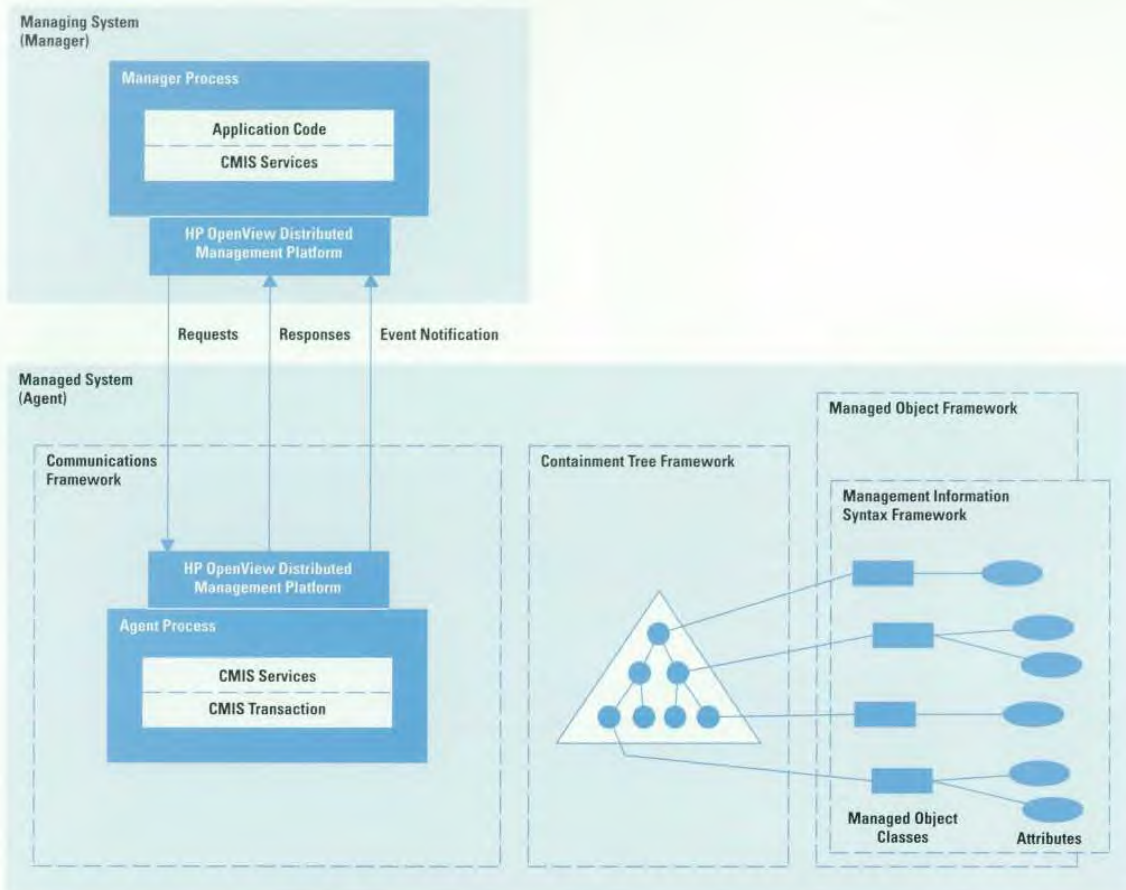
Fig. 6. Managed Object Toolkit frameworks.
