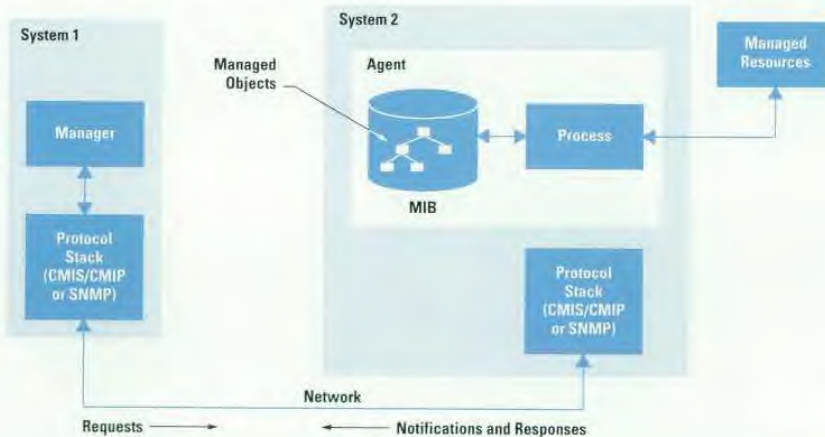
Fig. 1. The agent/manager model.
