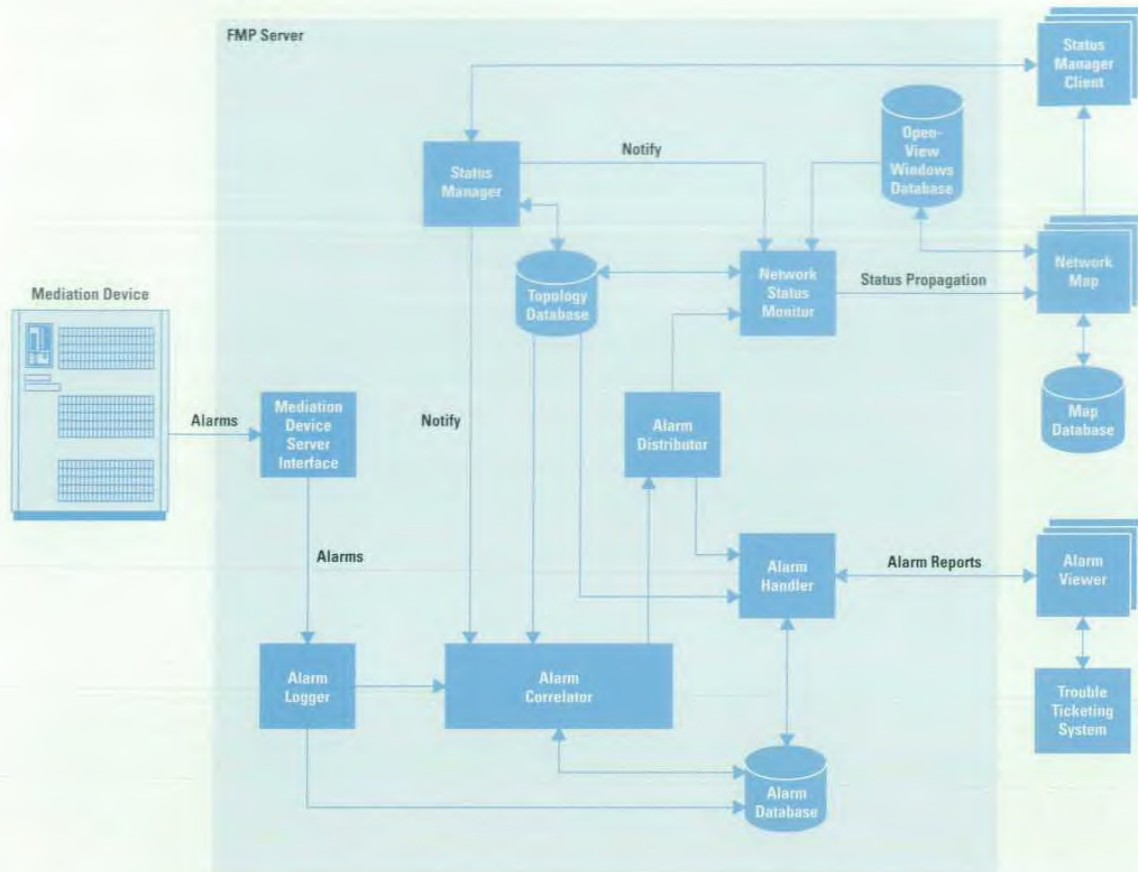
Fig. 7. FMP server functional block diagram.
