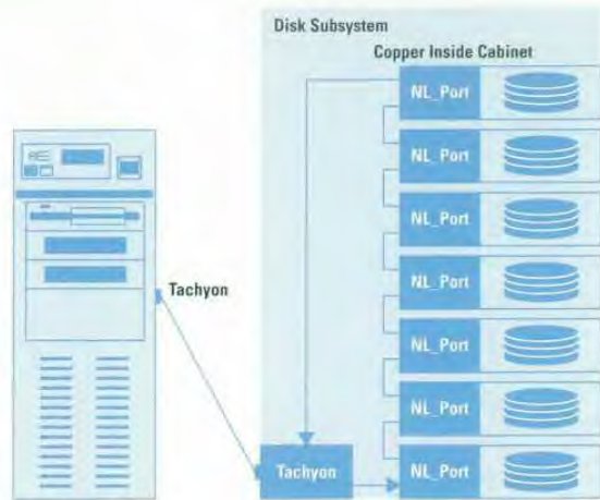
Fig. 4. A private disk loop.
