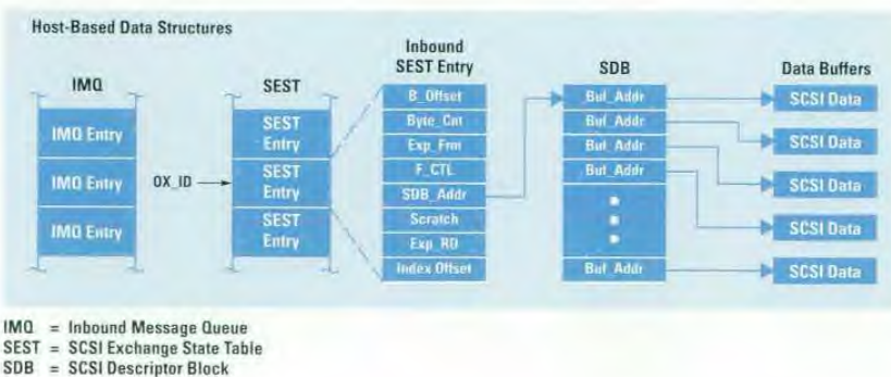
Fig. 9. FCP read exchange initiator host data structures.
