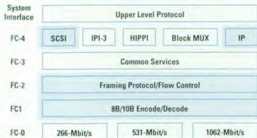
Fig. 7. Fibre Channel's five layers.
