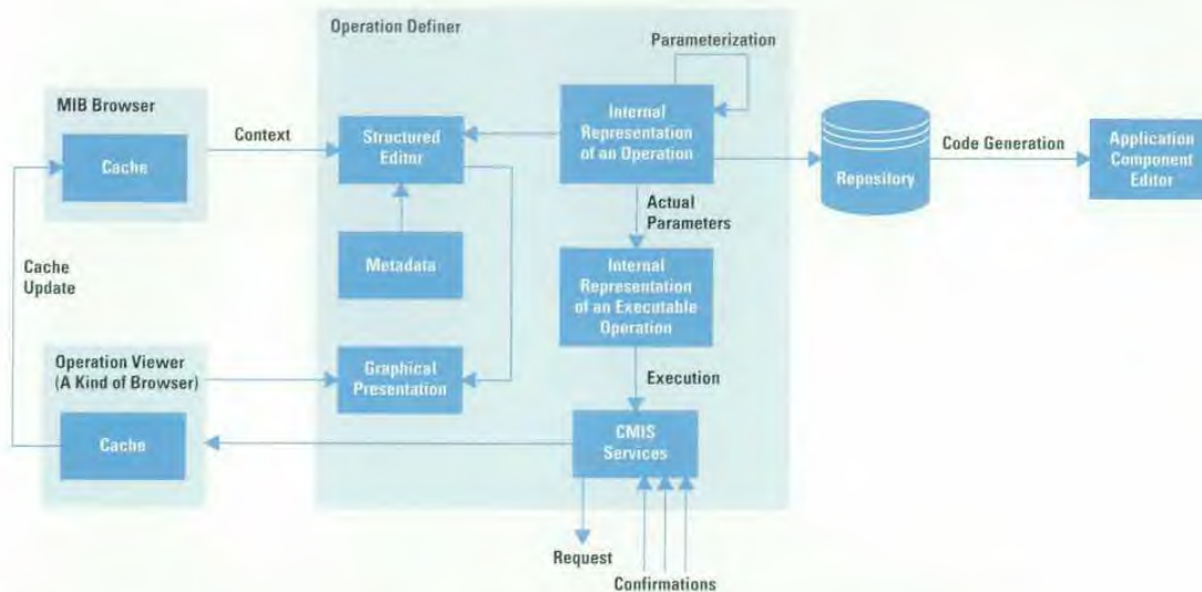
Fig. 5. The design of the operation definer.
