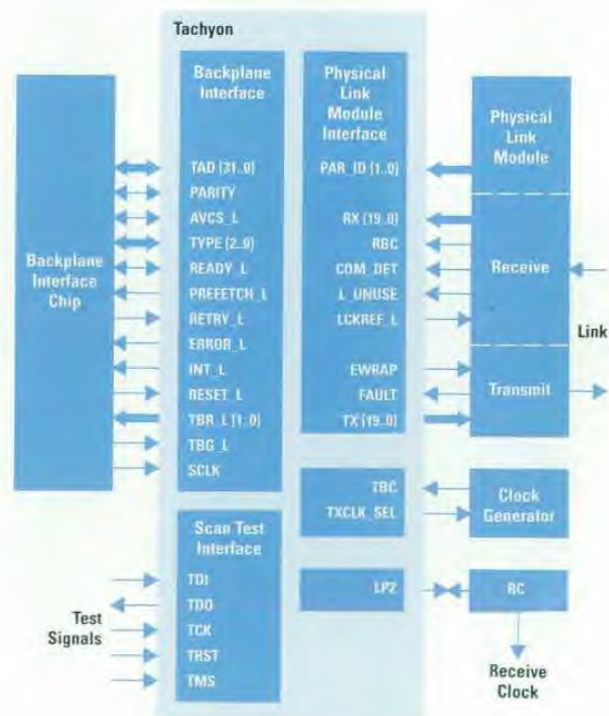
Fig. 13. Tachyon system interface.
