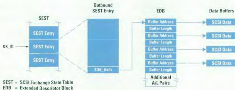
Fig. 11. FCP write exchange initiator host data structures.
