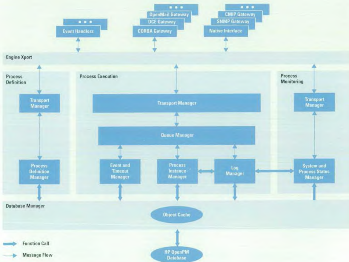
Fig. 3. Block diagram of the HP OpenPM engine.
