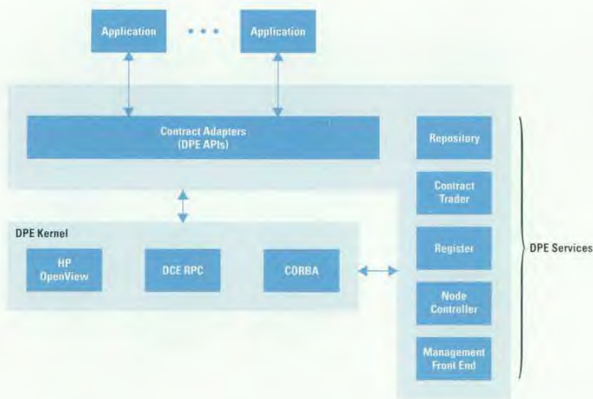
Fig. 2. Components of the DPE architecture.
