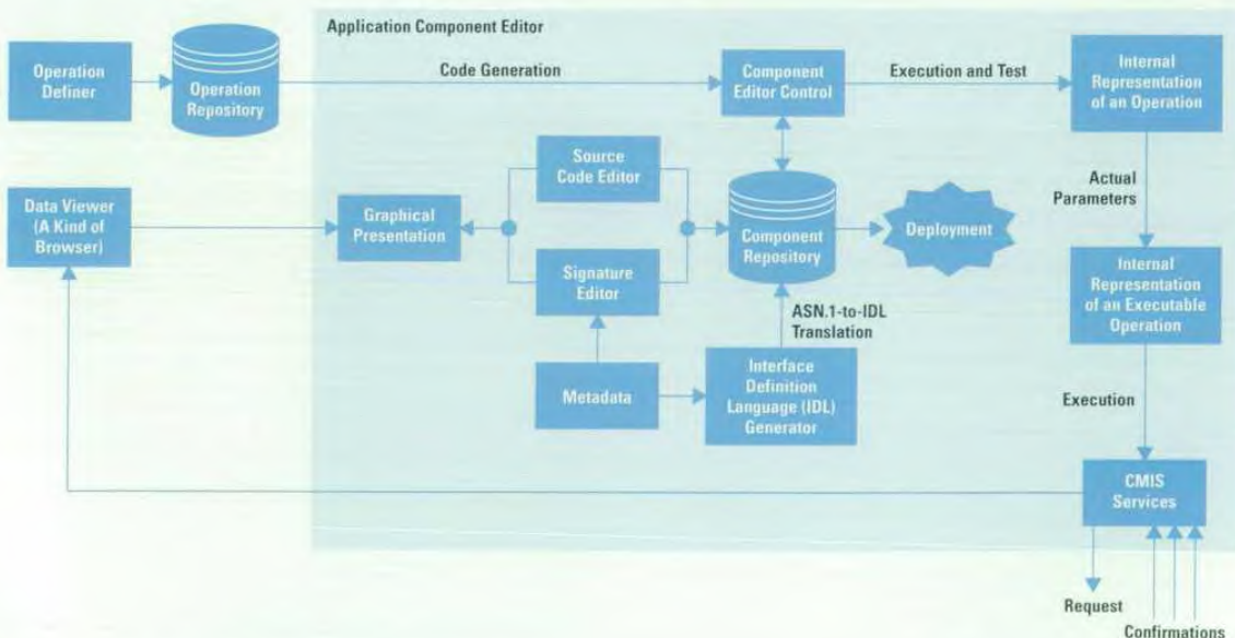
Fig. 7. The design of the application component editor.
