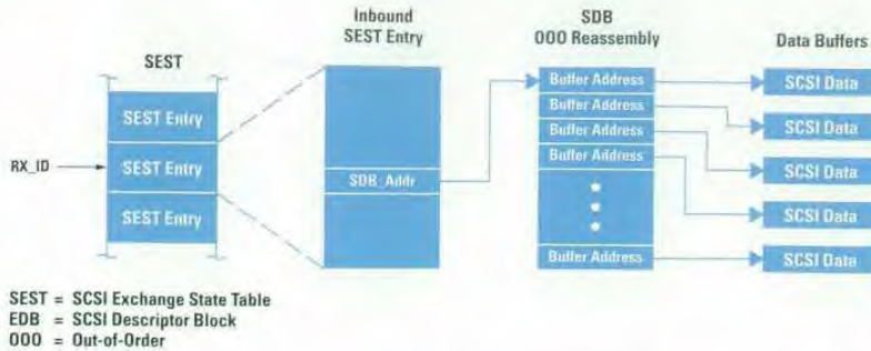
Fig. 12. FCP write exchange target host data structures.
