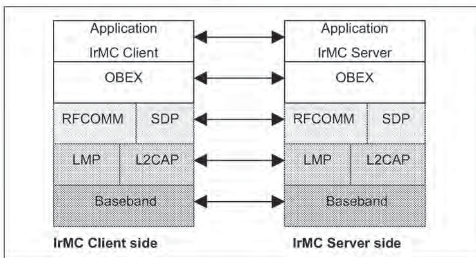
Figure 2.1: Protocol model
