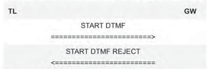
Figure 10.7: DTMF signalling, unsuccessful case
