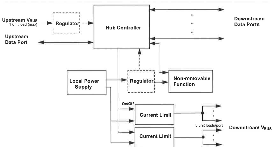
Figure 7-33. Compound Self-powered Hub
