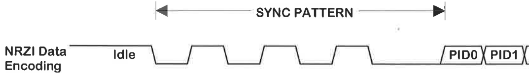
Figure 7-25. Sync Pattern
