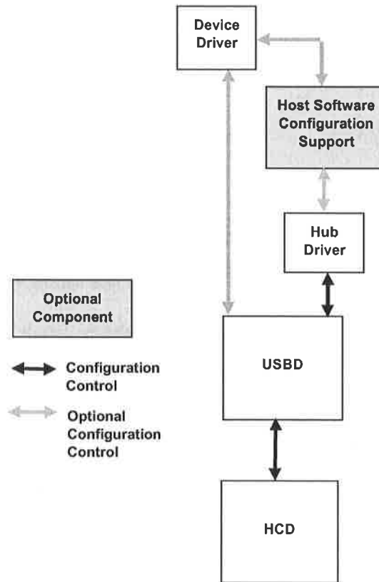
Figure 10-4. Configuration Interactions
