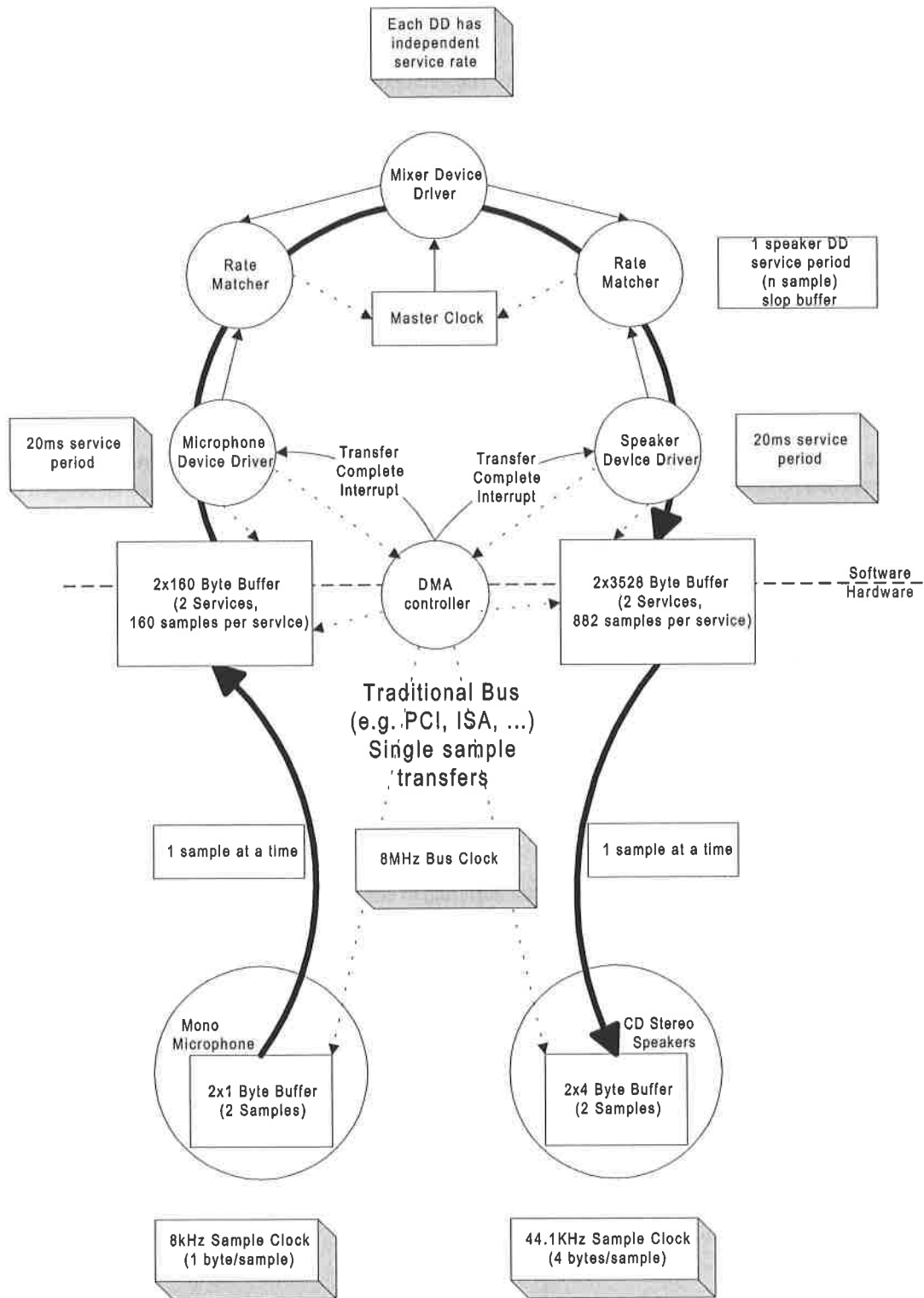
Figure 5-13. Non-USB Isochronous Example
