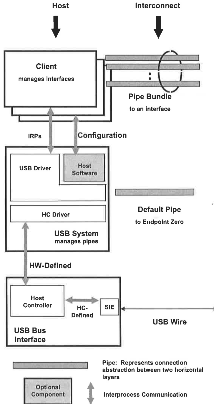
Figure 10-2. Host Communications
