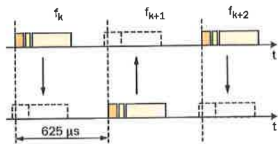
Figure 2 Frequency-hop/time-division-duplex channel.
