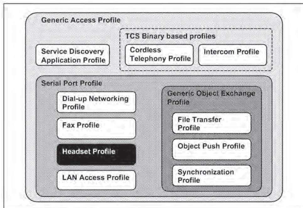
Figure 1.1: Bluetooth Profiles
