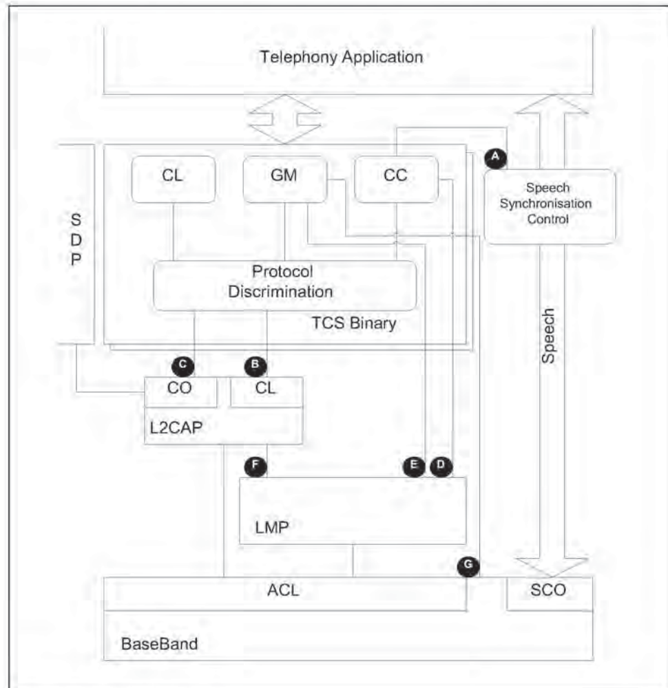
Figure 2.1: Protocol model
