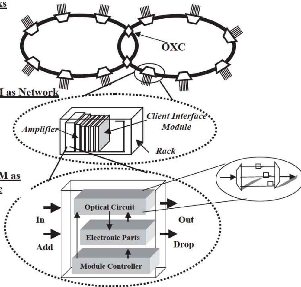
Fig. 1. ADM-as-optical-module is part of ADM network node which is positioned between two other network nodes of interconnected optical ring networks.
