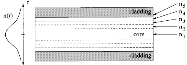
Fig. 6. Graded-index fiber.
