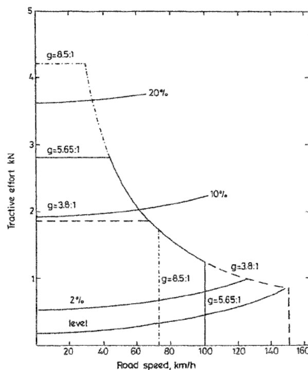
Fig 3 Tractive-effort and road-load curves for all-electric vehicle showing the effect of gear ratio
