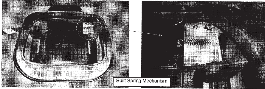
Seat Plate
