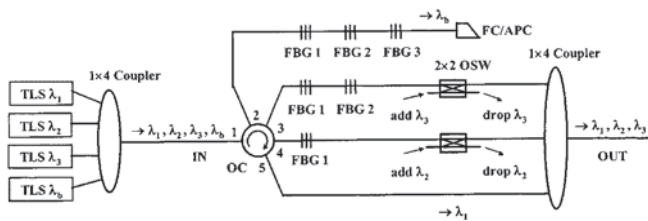
Fig. 2. Experimental setup of the proposed B-WADM. (TLS: Tunable light source.)
