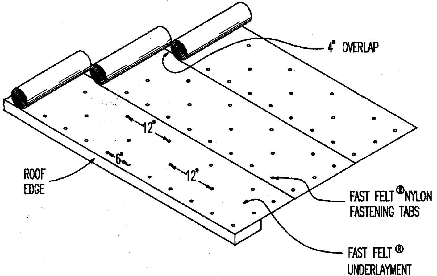
Detail "A" FAST FELT® NAIL FASTENING PATTERN
