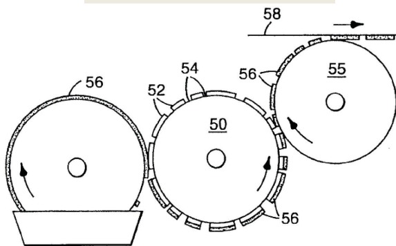
Fig. 4 PRIOR ART
