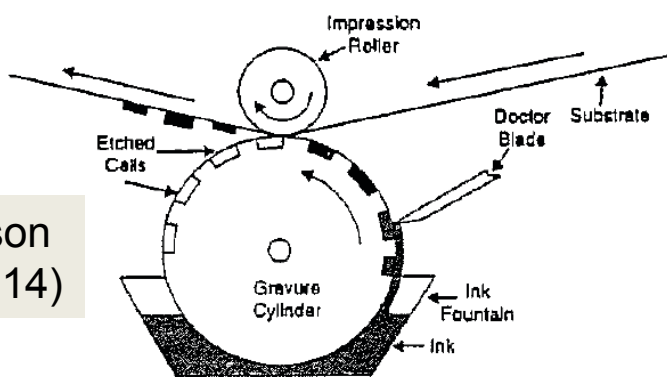
The gravure printing unit.
