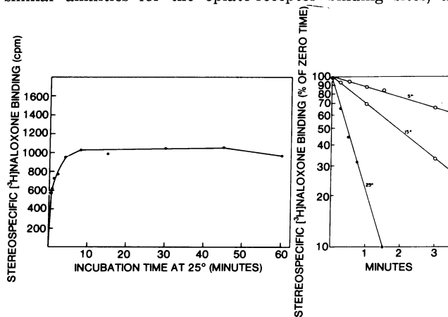
FIG. 5. Rate of stereospecific binding of [ ^3\text{H} ]naloxone at 25^\circ (left) and semilog plot of dissociation of bound [ ^3\text{H} ]naloxone from rat-brain homogenate at 5^\circ , 15^\circ , and 25^\circ (right). Left: Standard homogenates were incubated for intervals varying from 15 sec to 60 min with [ ^3\text{H} ]naloxone in the presence of 0.1 \mu\text{M} dextrorphan or 0.1 \mu\text{M} levorphanol at 25^\circ before cooling to 4^\circ . Samples were filtered immediately after cooling. Right: Brain homogenates were incubated for 15 min at 35^\circ with [ ^3\text{H} ]naloxone in the presence of 0.1 \mu\text{M} levorphanol or 0.1 \mu\text{M} dextrorphan in the standard binding assay. After cooling in an ice bath, nonradioactive naloxone ( 10 \mu\text{M} final concentration) was rapidly added and samples were filtered immediately (time 0) or allowed to incubate for various times at 5^\circ , 15^\circ , or 25^\circ before rapid cooling and filtration.
