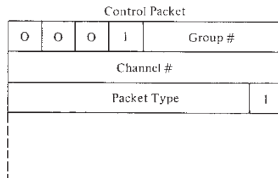
FIGURE 8.6 X.25 Layer 3 Packet Formats
