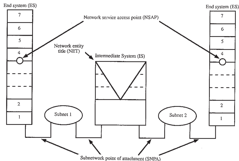
FIGURE 10.21 Network-Layer Addressing
