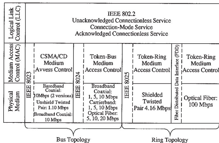
FIGURE 5.20 Local Area Network Standards
