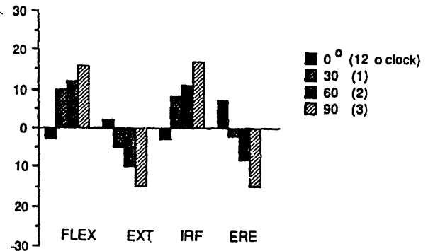
Fig 6 Effect of rotation of the elevated rim in type 1 liners—shell in malposition of 70° of abduction and 20° forward flexion. ROM of the plain liner is taken as the x axis. The bar graphs represent the increase or decrease in ROM of the ER liner in comparison with the plain liner. (A) Joint Medical 28 mm head +0 neck +20 ER liner. (B) PCA 26 mm head long neck and ER liner.
