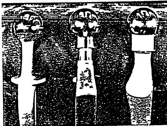
Fig 3 Head-neck geometry in modular vs nonmodular THAs tested (right to left) HD 2 HGP PCA. Note the increased neck diameter in the modular systems associated with cylindrical necks and most notably with flanges on some head components.
