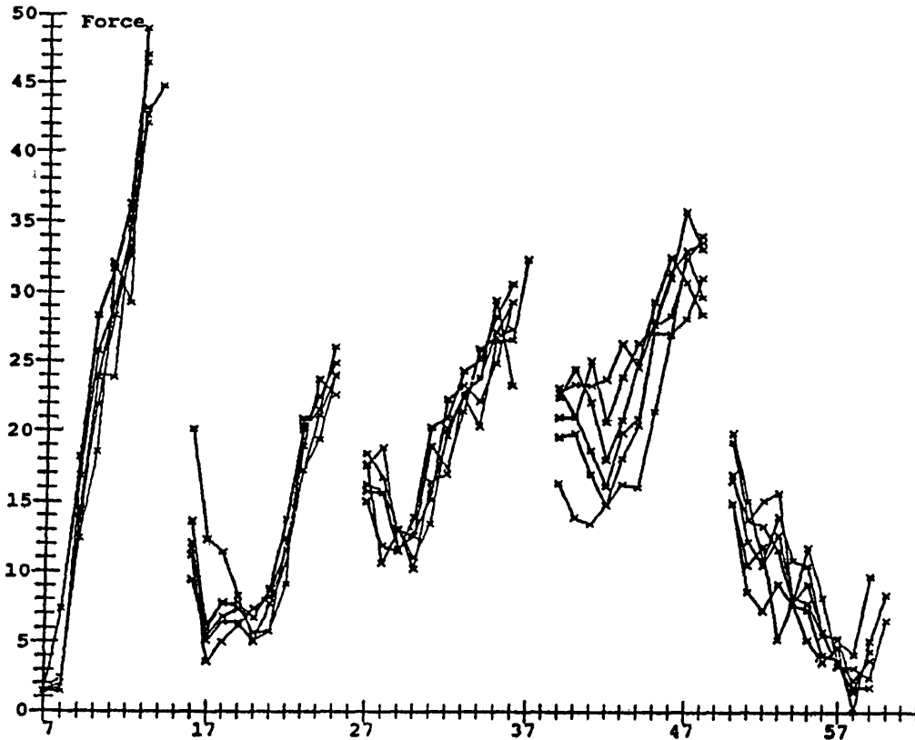
Fig 10 Cutting forces on cadaver dog bone. This figure shows a plot of the magnitude of the forces on the cutter tip for five typical rotational cuts. In this plot 40 force units correspond to one pound (0.45 kgf).
