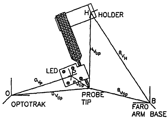
Fig 3 The probe tip with respect to the LED and the OPTOTRAK coordinate systems. The following notation is used: O OPTOTRAK coordinate system, P probe coordinate system, H probe holder coordinate system, B FARO arm base.
