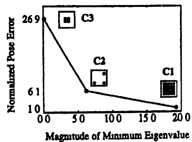
Fig 10 Accuracy vs minimum eigenvalue cube
