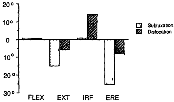
Fig 5 Type 2 liner standard position of 30° abduction and 20° forward flexion. The ROM of the plain liner is taken as the x axis. The bar graphs represent the increase or decrease in ROM of the ER liner in comparison with its corresponding plain liner. Changes in impingement/subluxation and dislocation are indicated. Shown here HGP with 26 mm head long neck and ER liner.
