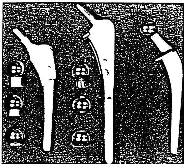
Fig 1 Femoral components tested shown together with their modular 26 mm head components (from left to right) PCA HGP and nonmodular HD 2. A flange or skirt is present on many longer neck modular head components. This flange fits over the end of the Morse taper of the femoral component and in effect widens the neck of the femoral component.
