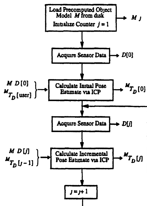
Fig 3 Tracking algorithm
