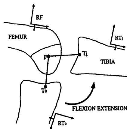
Fig 2 Attachment points of a graft F and T on the femur and the tibia respectively. During a flexion-extension of the knee the variation of the distance between F and T_0 T_j is called anisometry. If the trajectory of T belongs to a sphere centered in F the graft is perfectly isometric.
