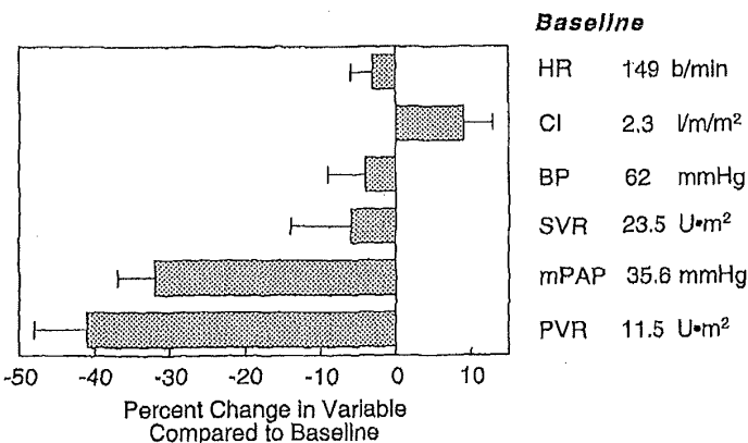
Figure 4. Percentage change in hemodynamic variables from baseline during 15 minutes of NO at 80 ppm in 9 patients with TAPVC. There is marked specificity for the pulmonary circulation.
