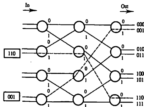
Figure 18.10 8 x 8 Banyan packet switching network.
