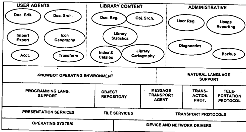
Figure 3 Personal Library System Structure
