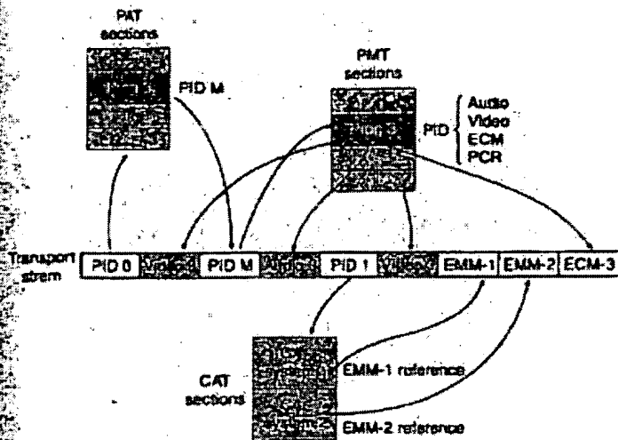
Fig. 5.3 Process by which the ECM and the EMM are found in the transport stream
