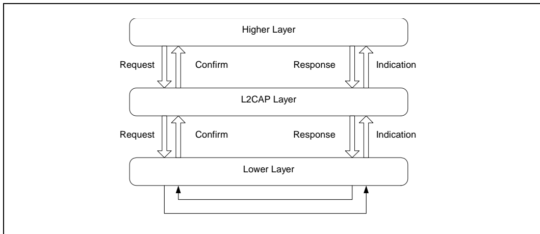
Figure 2.2: L2CAP Architecture
