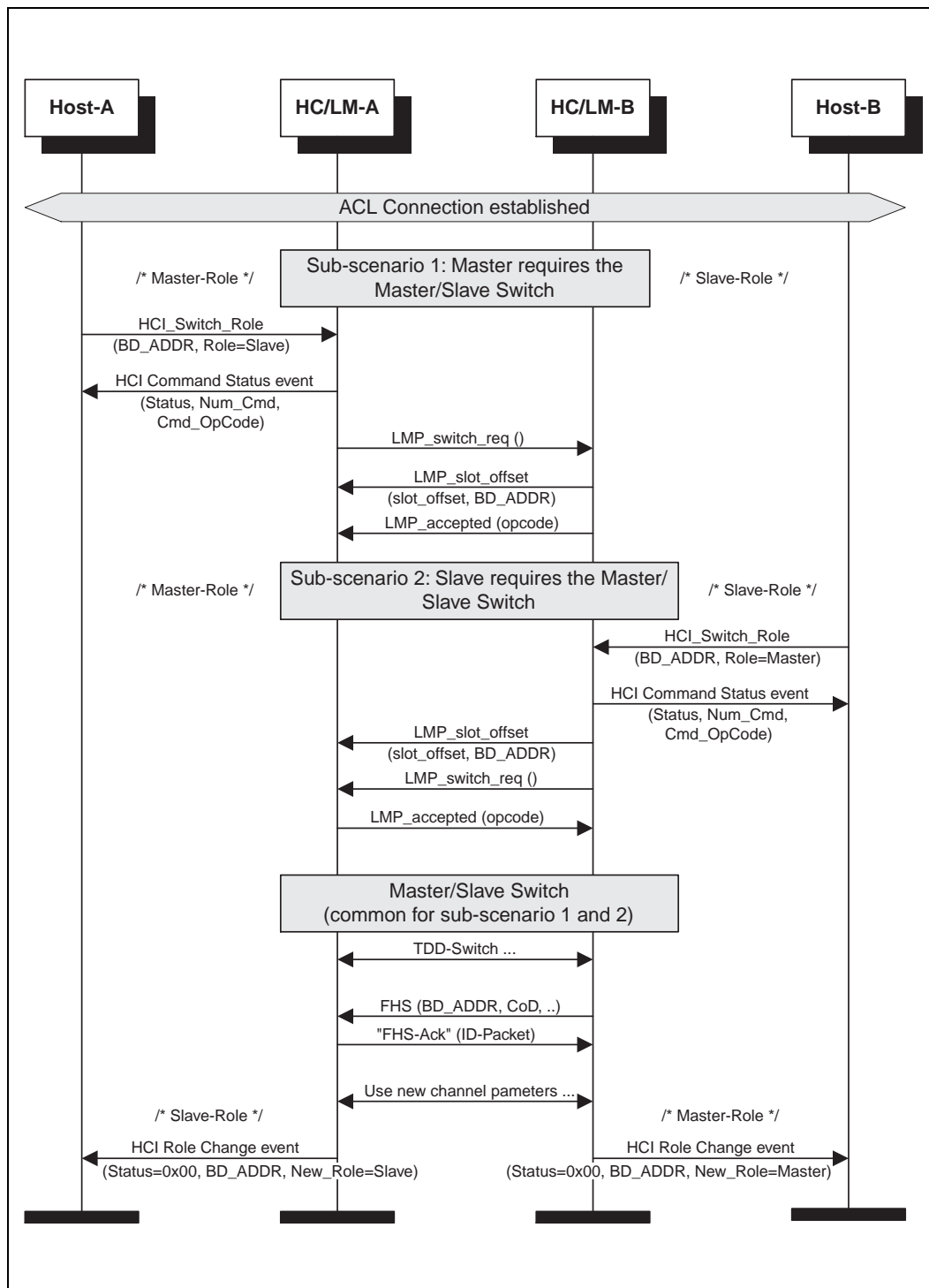
Figure 4.9: Switch Role
