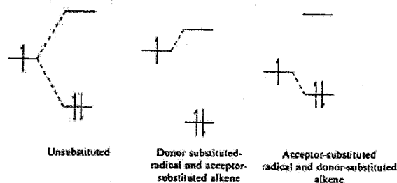
Fig. 12.5. Frontier orbital interactions between different combinations of substituted radicals and alkenes.
