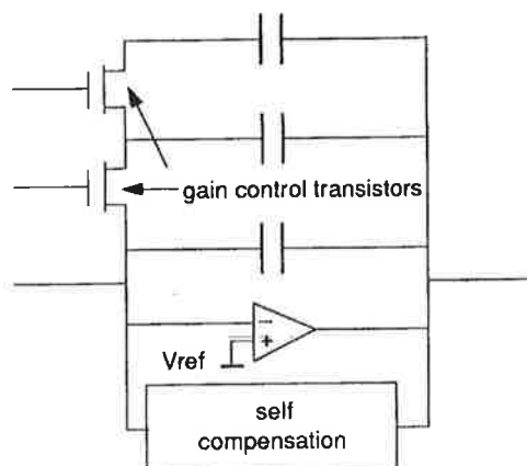
Figure 3. Integrator with programmable gain and self compensation
