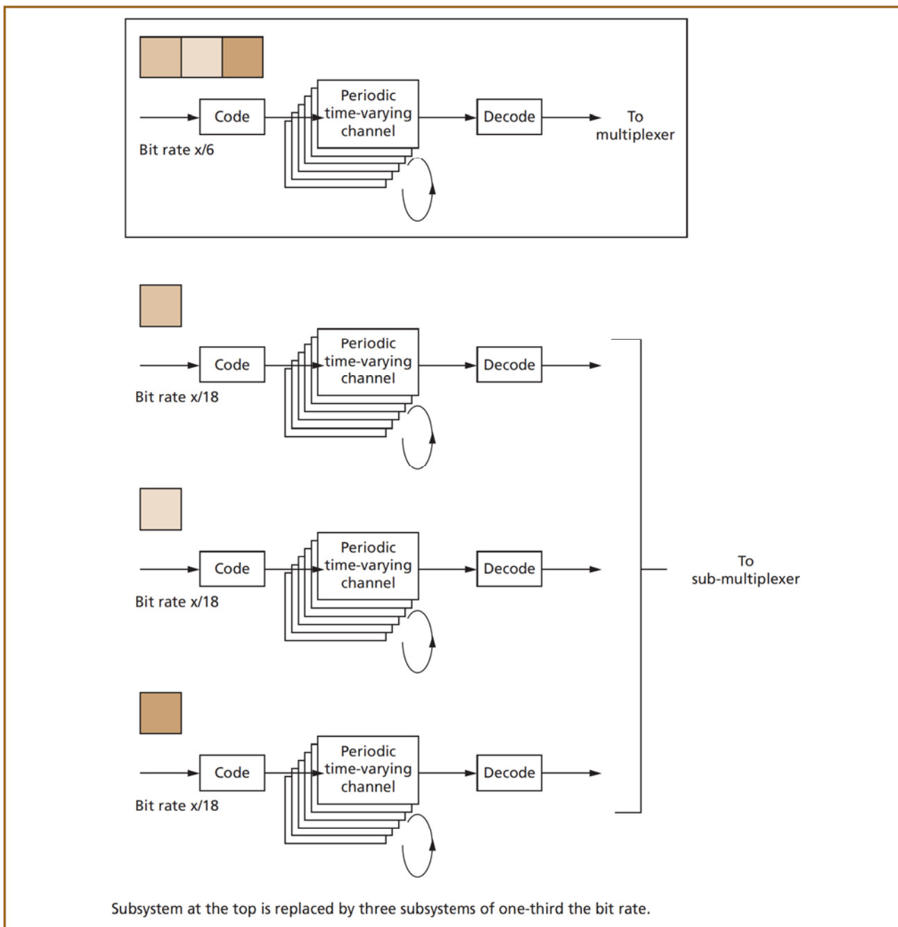
Figure 11. In parallel receiver processing, three time-varying channels run in parallel.
