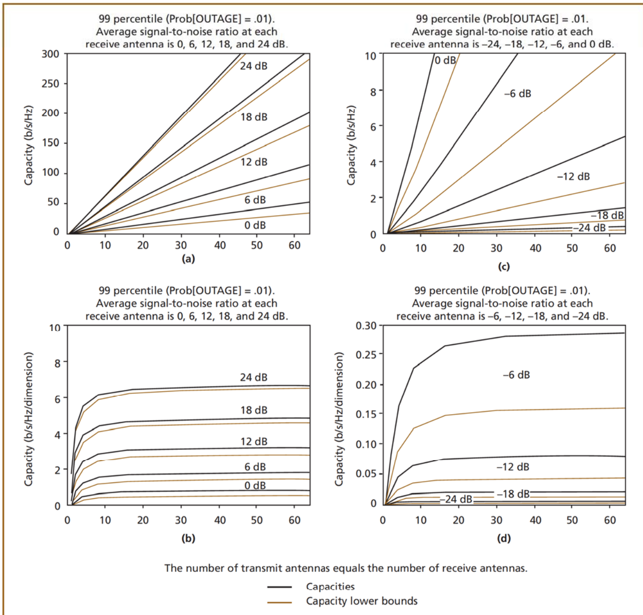
Figure 3(a). Capacity in b/s/Hz versus the number of antenna elements at each site.
