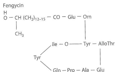
FIGURE 6.3 Structure fengycin.
