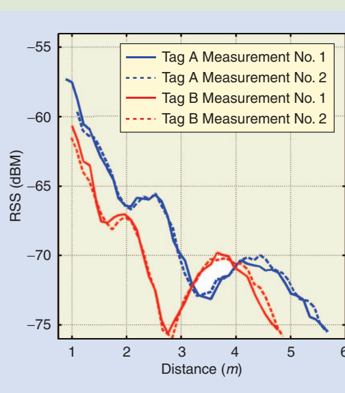
Figure S2. Multipath fading can cause large differences in field strength. The plot shows received signal strength versus distance in a direct line of sight situation. Tag B is placed 0.2 m below tag A.
