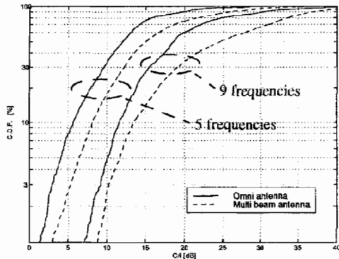
Figure 5. Downlink C/I with 9 and 5 frequency reuse in the exhibition hall for a system with omni antennas and multi beam antennas (6 beams) respectively.
