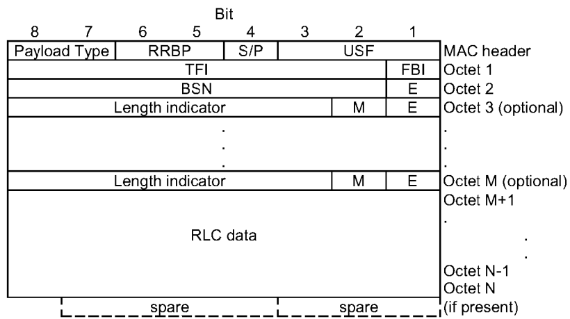
Figure 3: Downlink RLC data block with polling
