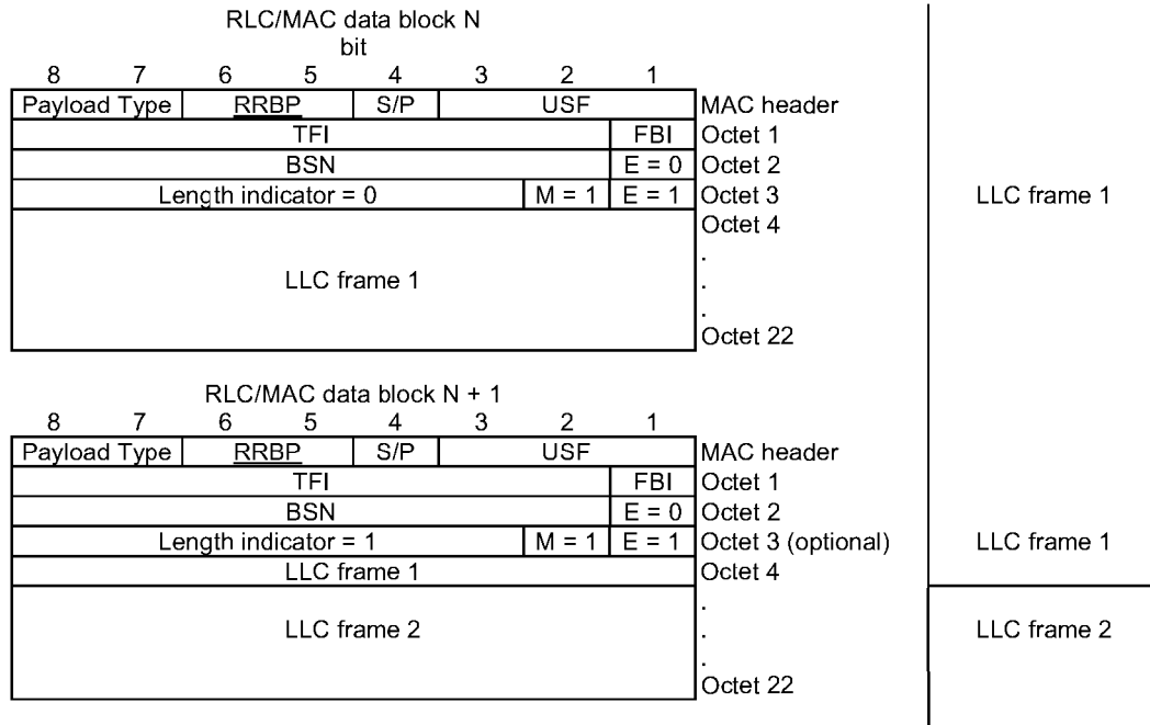
Figure B.2: Length indicator (LI) example
