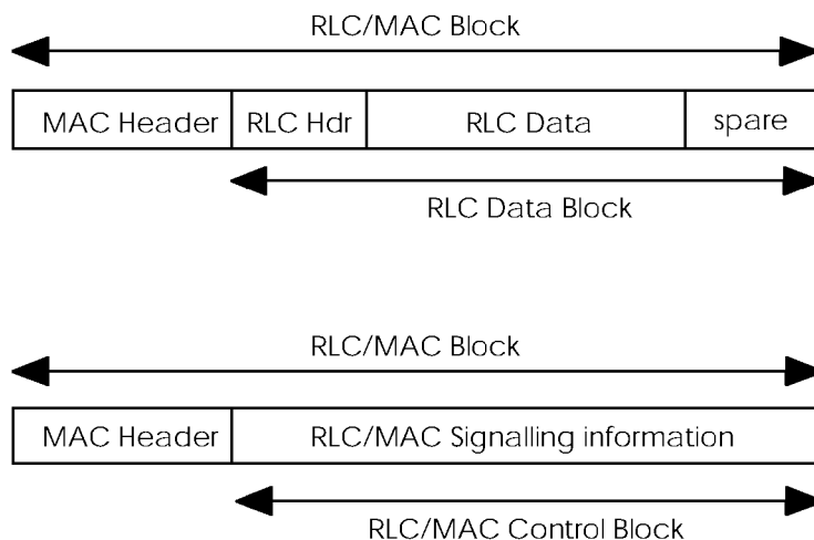
Figure 2: RLC/MAC block structure
