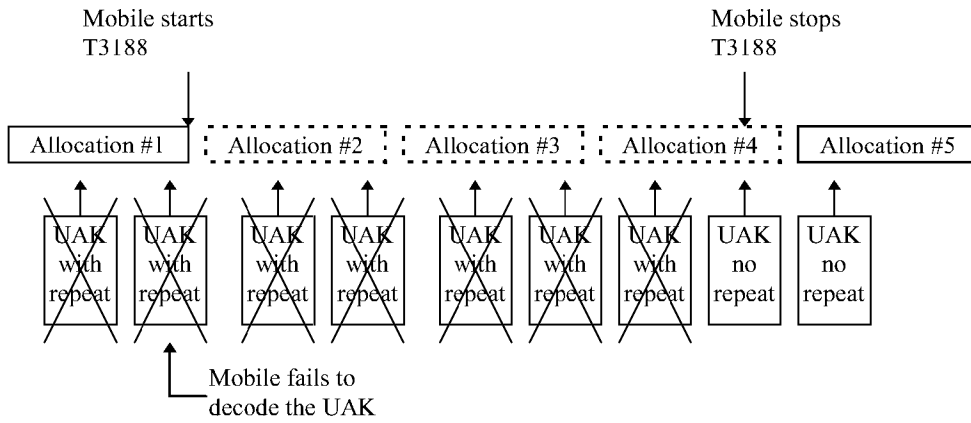
Figure E.3 Multiple Missed Uplink Ack/Nacks
