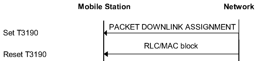
Figure C.2: TBF establishment initiated by the network
