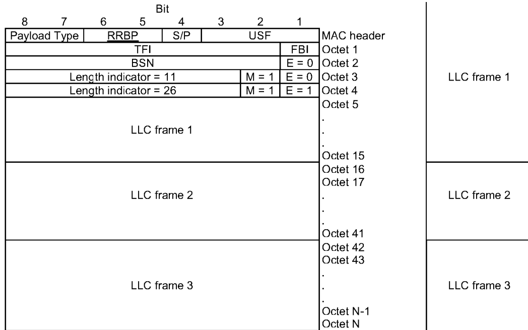
Figure B.1: Length indicator (LI) example
