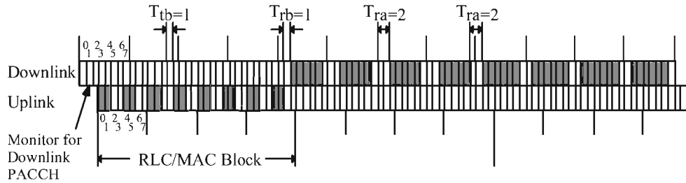
Figure D.15: Multislot Class 21 (Rx=6, Tx=4, Sum=NA), 4 timeslot uplink TBF, with a transition to a 6 timeslot downlink timeslot
